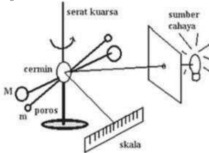
Gambar 3. Neraca Cavendish
