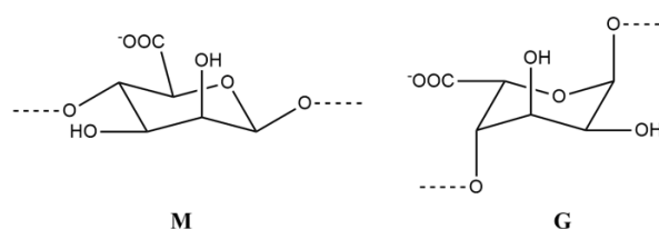
Figure 3. The monomers of alginate [50]
