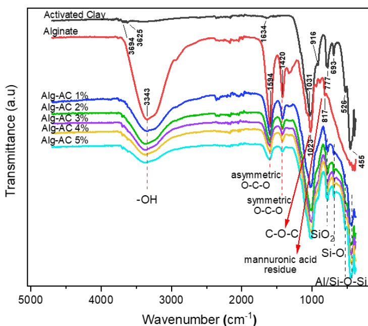
Figure 4. FTIR spectra of activated natural clay, alginate, and alginate-clay composite beads (Ag-AC 1-5%)
