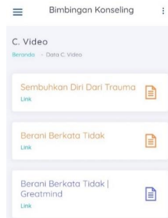
Gambar 4. Halaman Video
