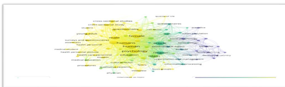
Gambar 10. Overlay Visualization
