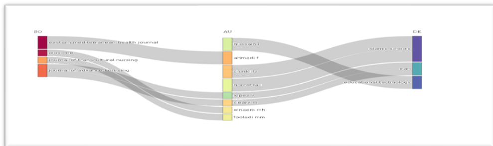
Gambar 7. Three-Field Plot
