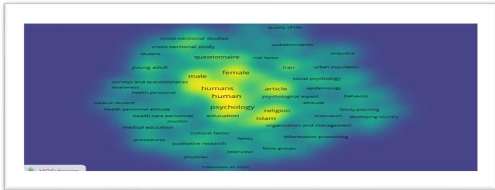
Gambar 11. Density Visualization
