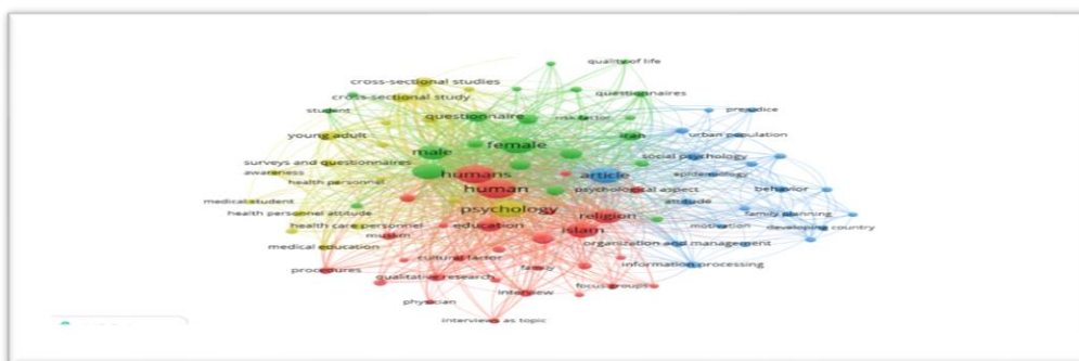
Gambar 9. Network Visualization
